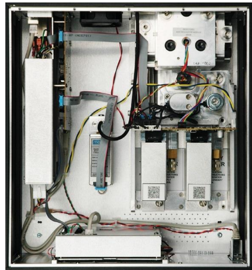
Chassis assembly.
