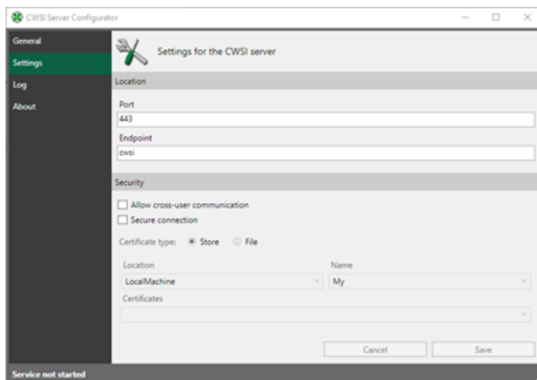
Figure 5: CWSI Server Setting Page
