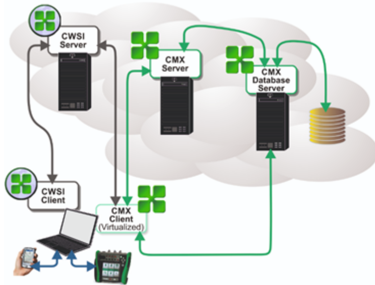
Figure 1: CWSI Client and Server
